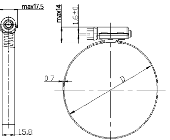
HOS 15.8 THICKNESS:0.7mm BANDWIDTH:15.8mm
