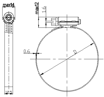
HOS 12.7 THICKNESS:0.6mm BANDWIDTH:12.7mm
