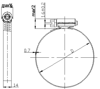
HOS 14.2 THICKNESS:0.7mm BANDWIDTH:14.2mm
